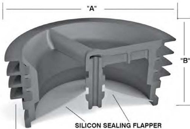
SILICON GASKET FLEXES .100" TO FIT DIAMETER
