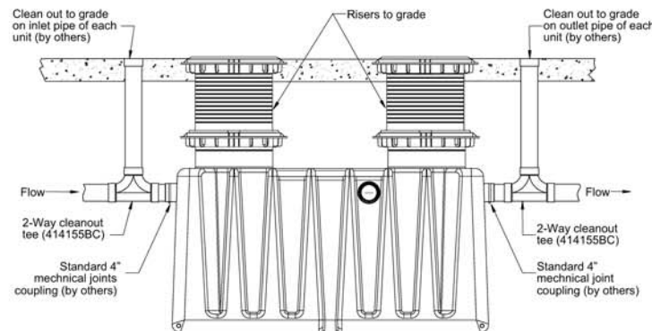
SIDE VIEW DETAIL
